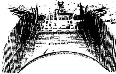
The stilling basin of the Willow Creek structure near Pierce (pictured under construction) will catch water which comes through the 6' diameter spillway tube. It will slow the water going into the stream so it does no damage.
