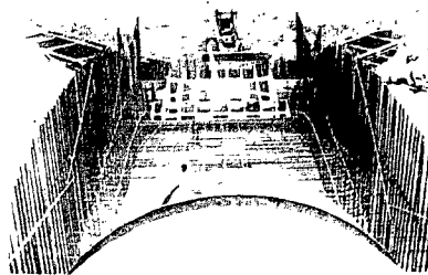
The stilling basin of the Willow Creek structure near Pierce (pictured under construction) will catch water which comes through the 6 diameter spillway tube. It will slow the water going into the stream so it does no damage.
